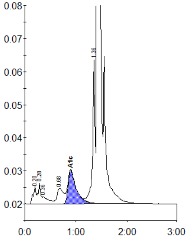
Peak table - ID: 10515532
